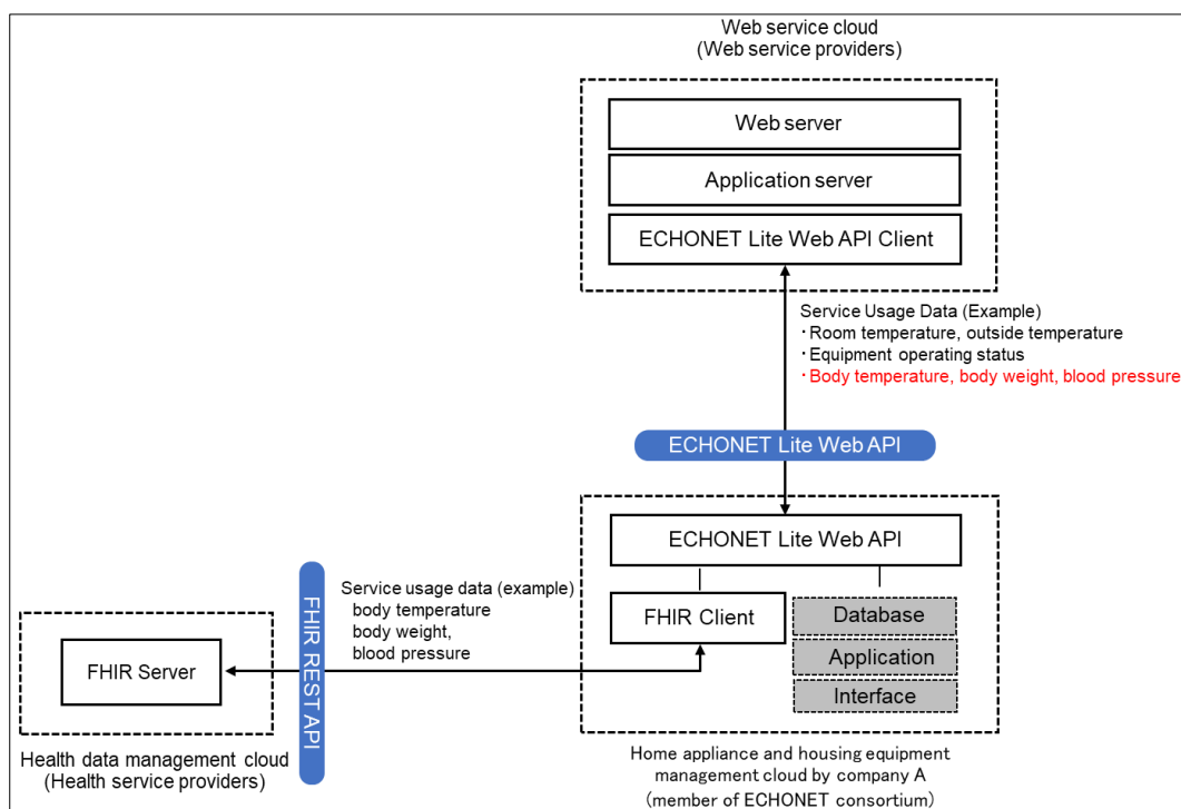
Figure 10 PCHA—Structure on ECHONET Consortium data linkage
