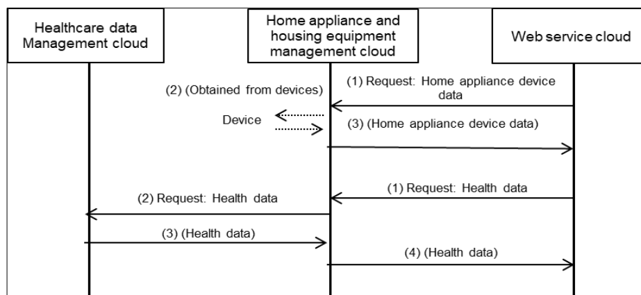
Figure 12 Health and home appliance device data acquisition from Web service cloud
